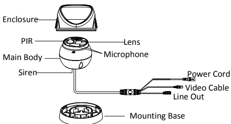
Figure 1-2 Overview of Type II Camera
