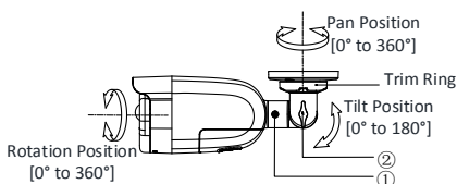
Figure 2-2 3-Axis Adjustment
