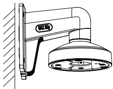
Figure 2-14 Fix Wall Mount
