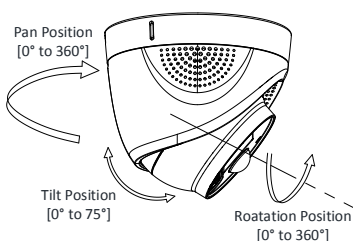
Figure 2-10 3-Axis Adjustment
